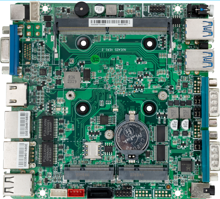
CX-J4125-2C-2L
